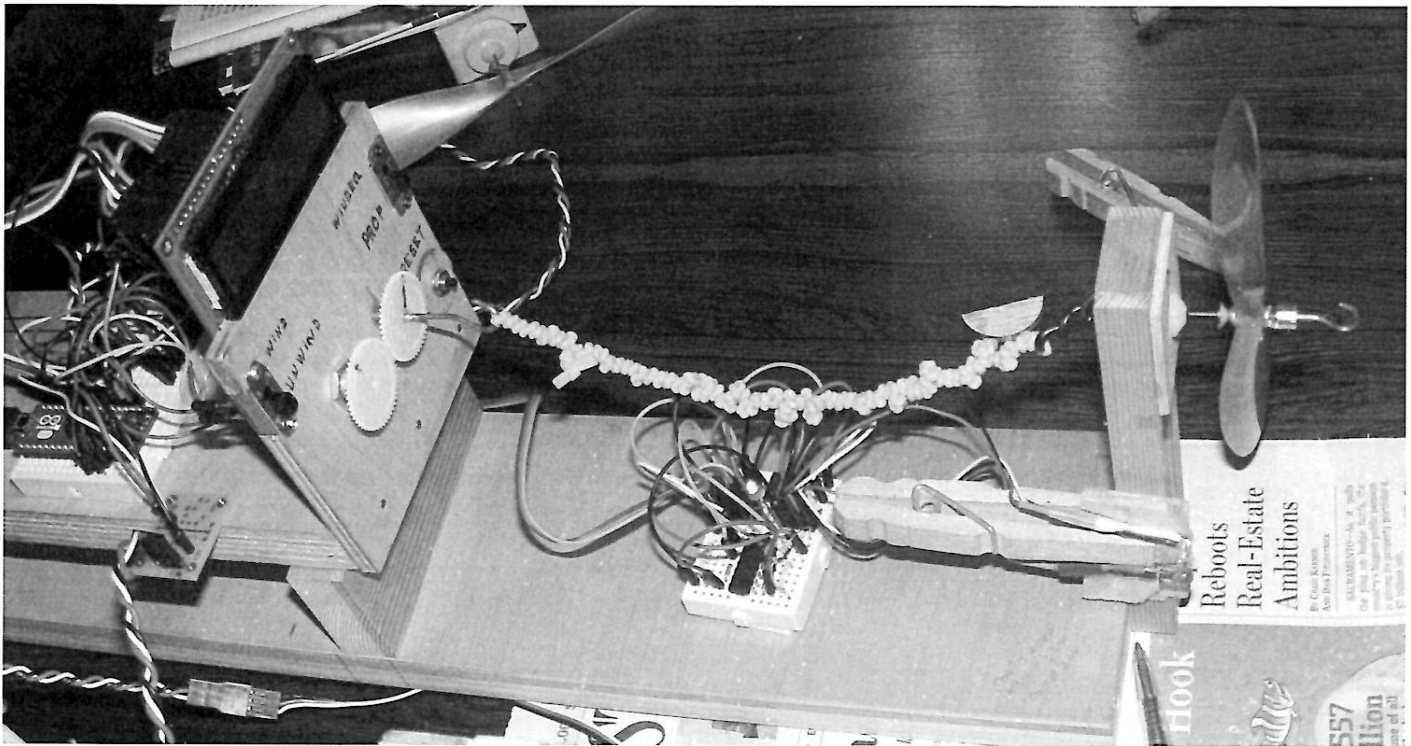
NO, THIS ISN'T A "SAG" TEST. IT'S A STOP ACTION SHOT OF A RAPIDLY SPINNING MOTOR WITH A LARGE STANDING WAVE. THAT "O" RING MAY HAVE CLIMBED OFF CENTER ON THE HOOK. THE PROP HAS FRONT LOOP TO MINIMISE INSERTION LOSSES OF TENSION & TORQUE.
