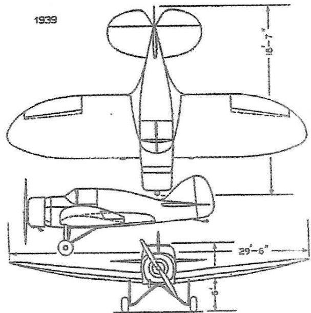
Figure 3. Culver Dart GW 3-View
