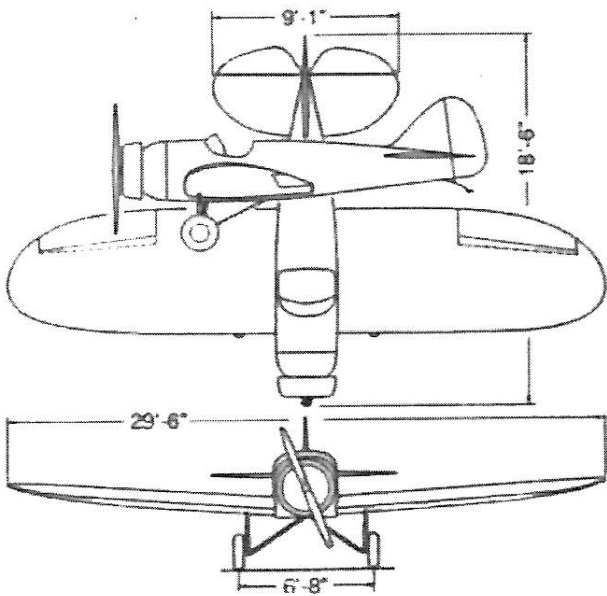
Copy of page 295 from The Aircraft Yearbook for 1937, a publication of the Aeronautical Chamber of Commerce of America, Inc., New York. The original of this three view by Harry Pack is presently owned by Bill Hannan and was used to provide the outline for the plans of the Monoprep Peanut.
